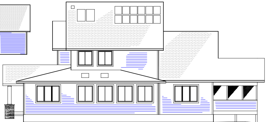
SOUTH
